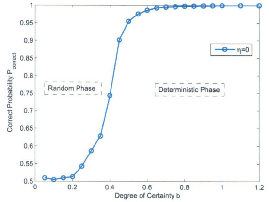
Fig. 9. P_{\text{correct}} vs. b with \eta = 0 .
